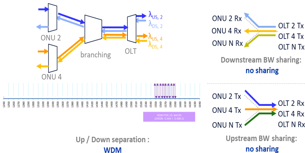
Figure F.1-3: WDM PON: Up- and Downstream Separation by WDM, without Up- and Downstream Bandwidth Sharing
