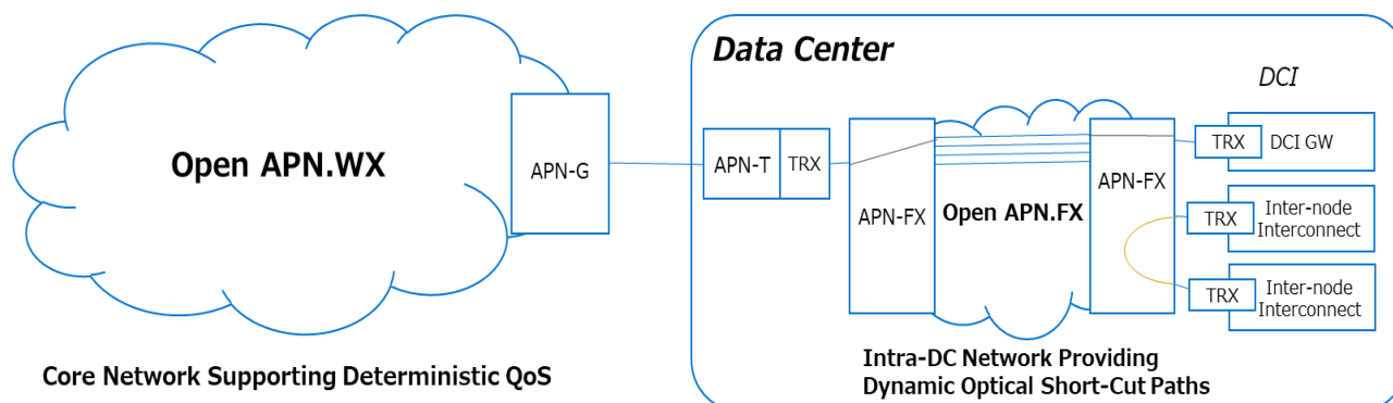
Figure I.1-6: Open APN.FX as Intra-DC Network
