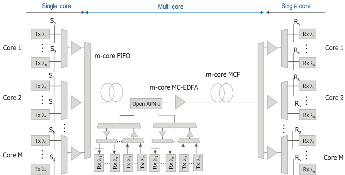
Figure B.3-4: The Multicore Fiber Transmission Reference Model
