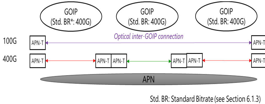
Figure Error! Use the Home tab to apply 見出し 3 to the text that you want to appear here.-1: Inter-GOIP Connections
