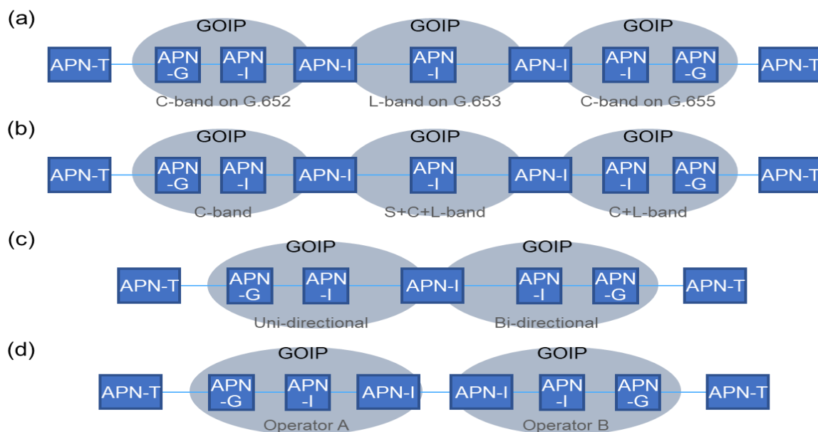
Figure 6.1.5-3: End-to-end Direct Connection across Multiple GOIPs Realized by Adaptation Function of APN-I
