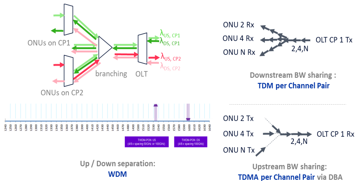
Figure F.1-4: TWDM PON: Up- and Downstream Separation by WDM, Up- and Downstream Bandwidth Sharing by TDM(A) per Channel Pair
