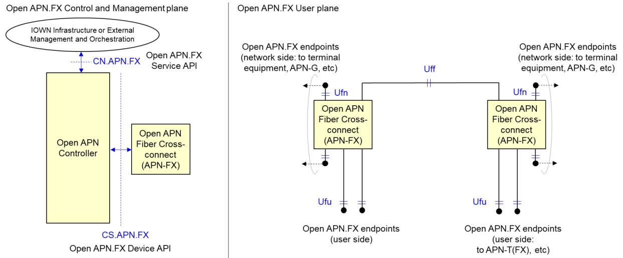
Figure Error! Use the Home tab to apply 見出L 3 to the text that you want to appear here.-1: Open APN.FX High-level Reference Architecture for PtP Fiber Path Services
