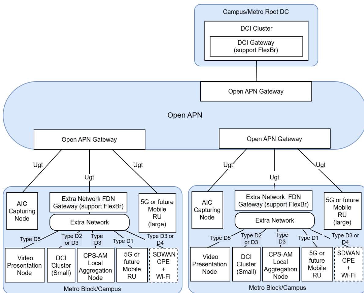
Figure A.3-1: Converged Network Service for Campus/Town/Metro
