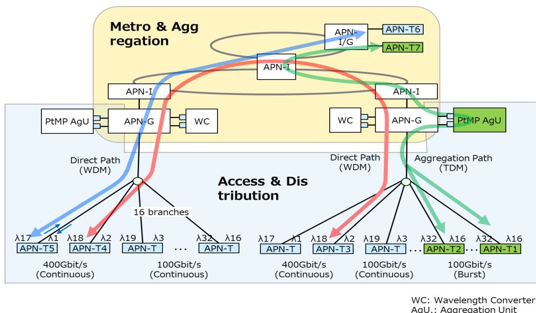
Figure F.2-1: Fiber Topology Example
