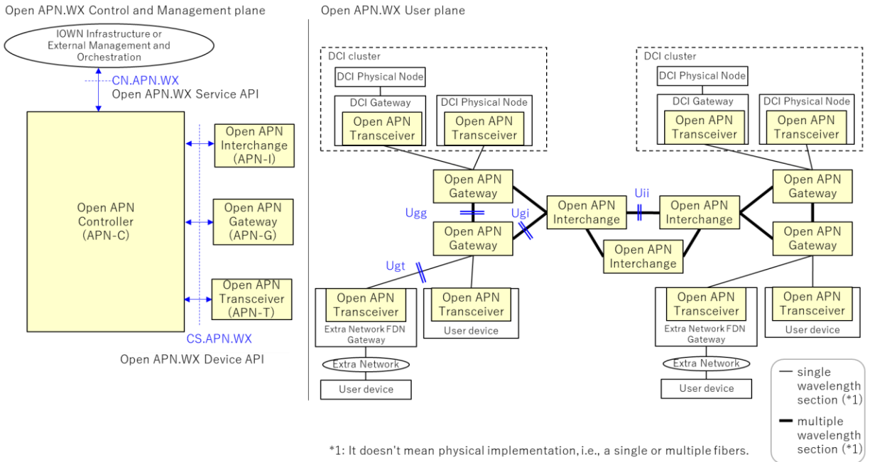
Figure Error! Use the Home tab to apply 見出し 2 to the text that you want to appear here.-1: Open APN.WX High-level Reference Architecture for PtMP Wavelength Path Services
