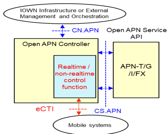
Figure Error! Use the Home tab to apply 見出し 3 to the text that you want to appear here.-1: Example of Controller Configuration for eCTI
