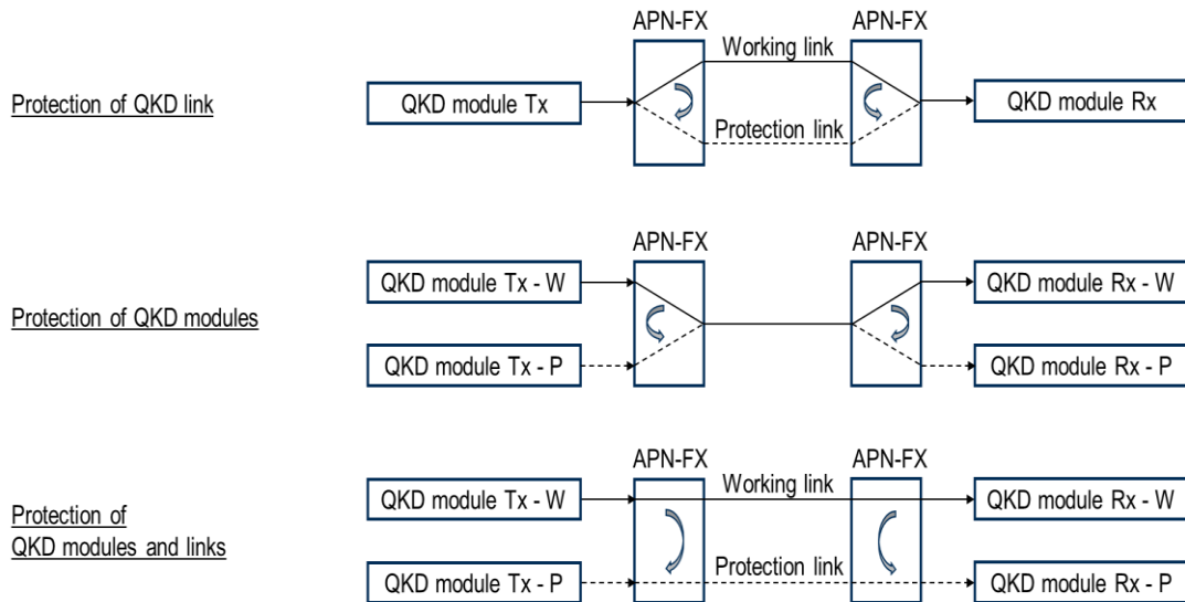
Figure J.3-4: Enhanced resilience through protection of QKD modules and/or links
