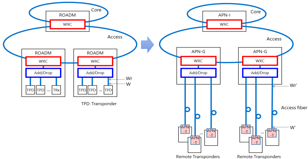
Figure 6.2-2: Relationship between ROADM and Open APN.WX Function Blocks
