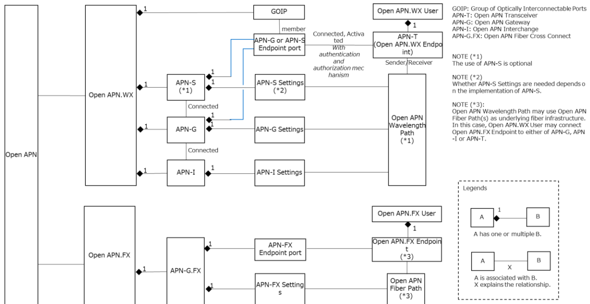
Figure 3.3-1: Object Model for Open APN Control Plane Service
