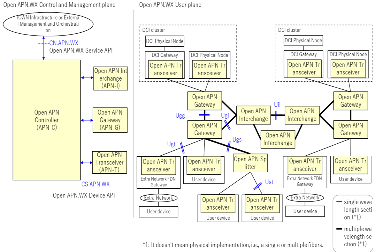
Figure 3.1.1-1: Open APN.WX High-level Reference Architecture for PtP Wavelength Path Services
