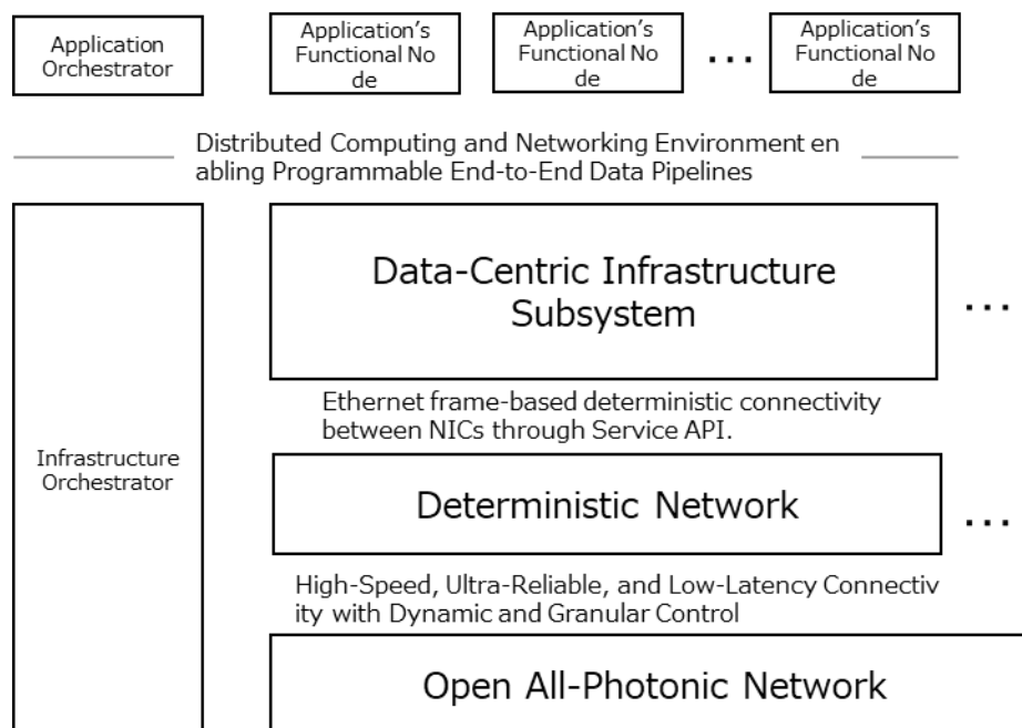
Figure 1.2-1: IOWN Global Forum Overall Architecture
