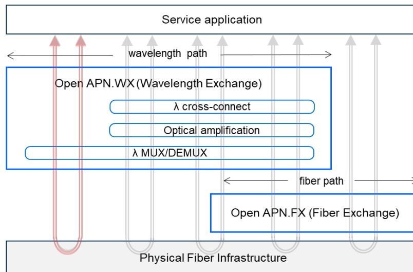
Figure 6.5-2: Layered structure view of Open APN service paths
