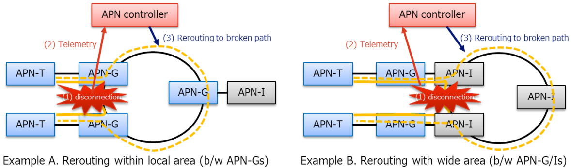
Figure D.2-1: Real-time Control for Resilient Network
