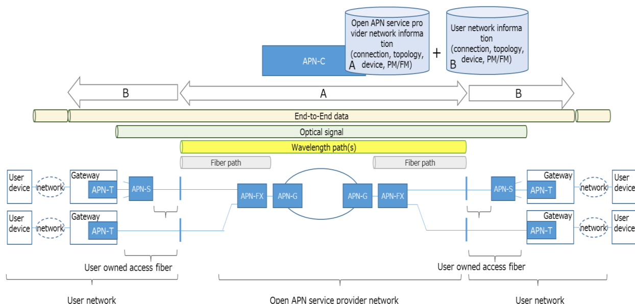
Figure 5.1-1: An Example Control and Management Scope of APN-C
