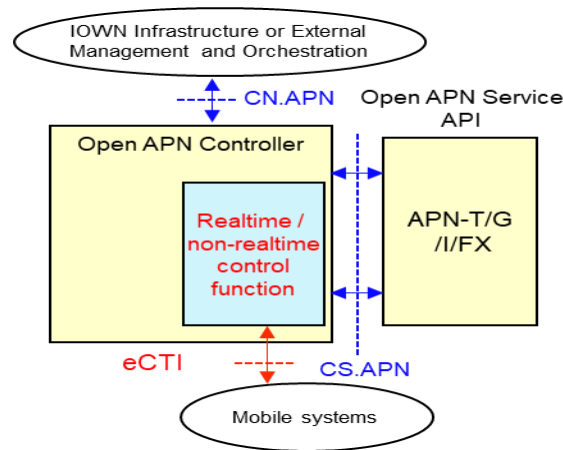
Figure 5.5.1-1: Example of Controller Configuration for eCTI
