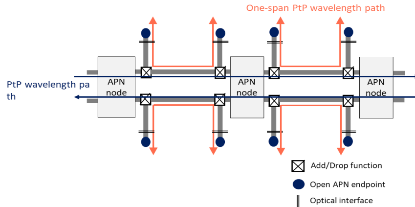
Figure 6.5-1: System configuration view of one-span PtP wavelength path
