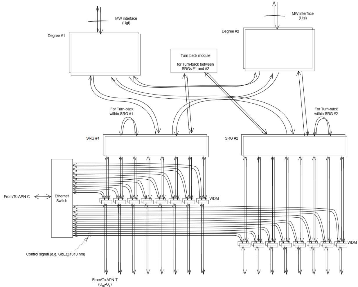
Figure C.2-2: Implementation Example of APN-G (2)
