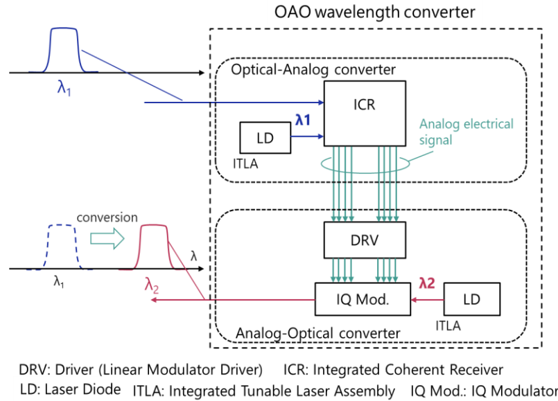
Figure B.3-10: Conversion principle of the OAO conversion
