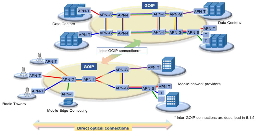
Figure 6.1.1-1: Schematic Diagram of GOIP
