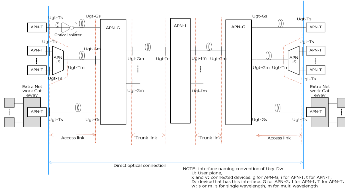
Figure 6.2-1: Architectural Diagram of Open APN.WX within a GOIP
