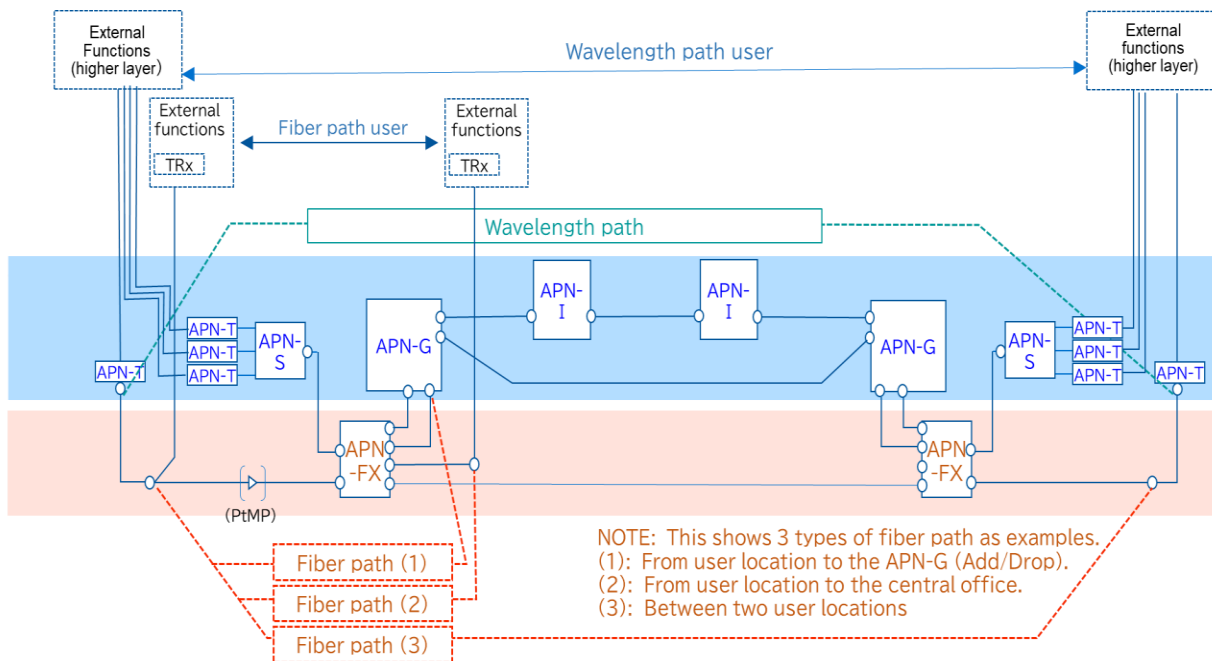
Figure 3.1.2-2: Example of the Relationship between Open APN.WX and Open APN.FX
