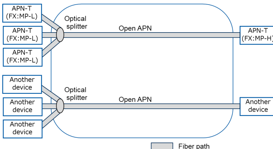
Figure 2.1.4-1: Point to Multi-point Fiber Path Service
