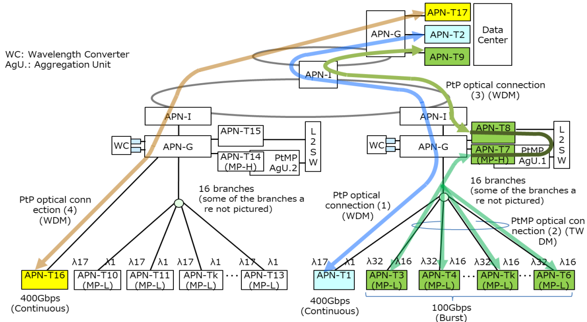
Figure F.3-1: An Example of Configuration Image of WDM PtP and PtMP Co-existence System
