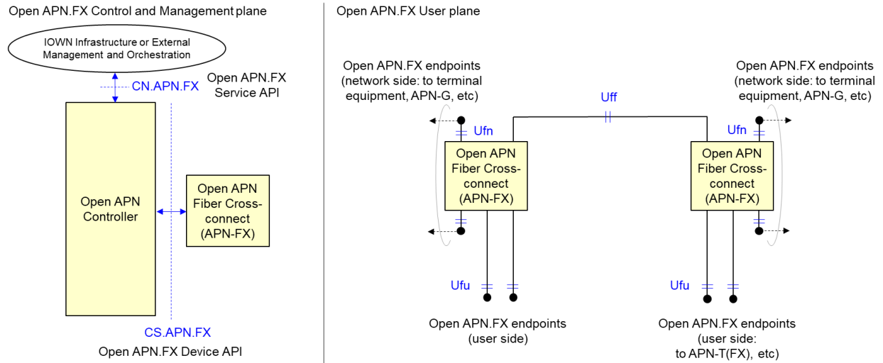
Figure 3.1.2-1: Open APN.FX High-level Reference Architecture for PtP Fiber Path Services
