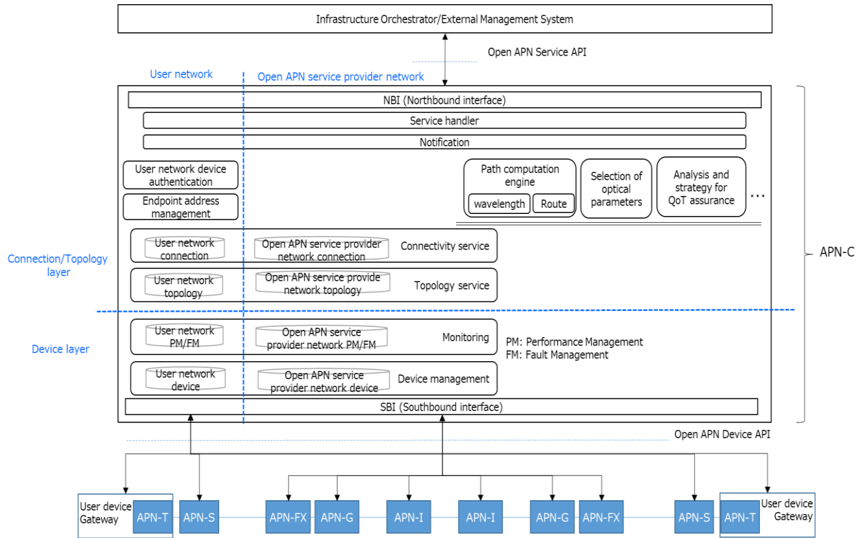
Figure 5.2-1: An Example Reference of APN-C Functional Model
