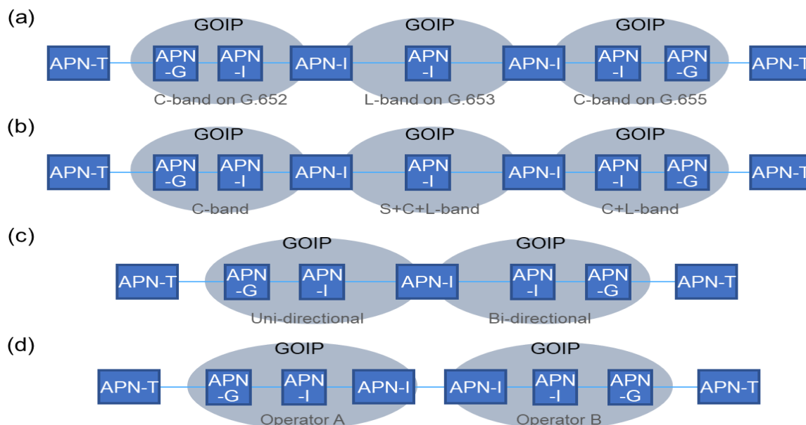
Figure 6.1.5-3: End-to-end Direct Connection across Multiple GOIPs Realized by Wavelength Conversion Function of APN-I
