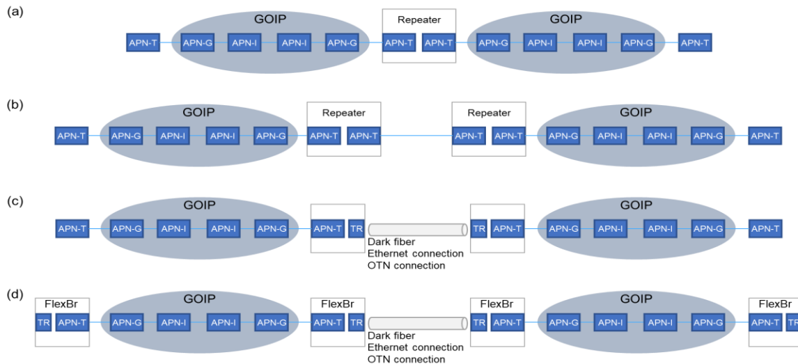
Figure 6.1.5-2: Direct Accommodation of User Data across Multiple GOIPs
