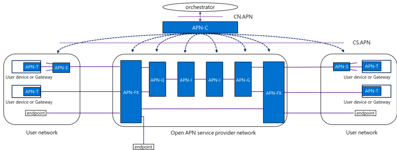
Figure 3.4-1: Example Network Reference Model
