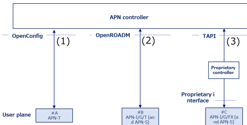
Figure 5.3-1: Recommendation Set of Southbound Interfaces (SBIs) for APN-C
