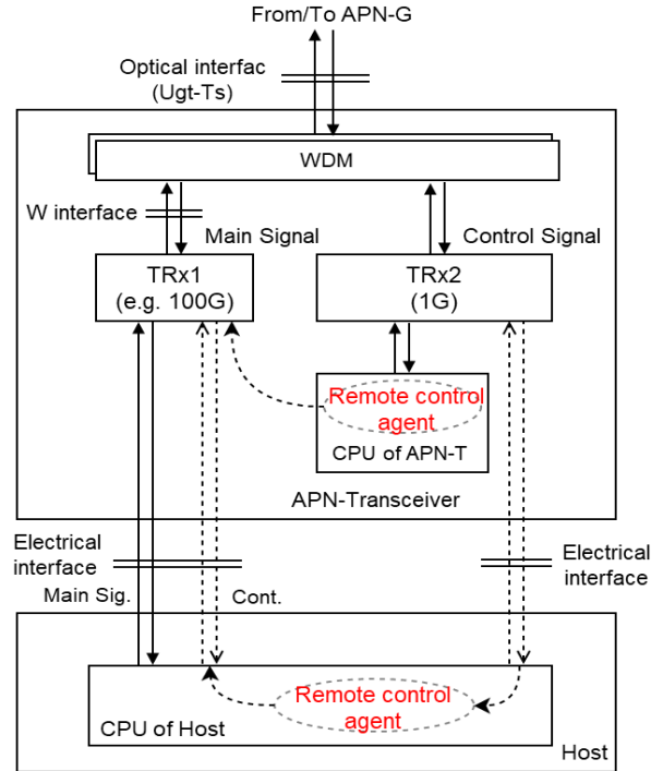
Figure C.3-2: Implementation Example of Integrated APN-T into Single Module
