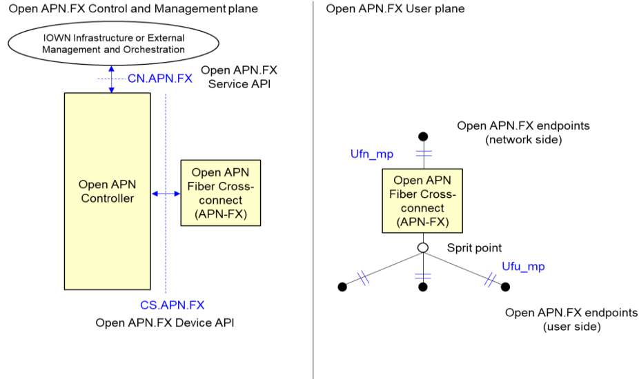
Figure 3.2-2: Open APN.FX High-level Reference Architecture for PtMP Fiber Path Services
