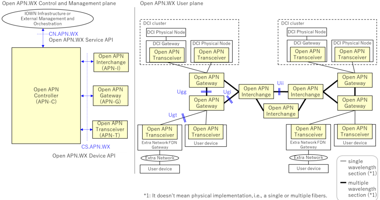
Figure 3.2-1: Open APN.WX High-level Reference Architecture for PtMP Wavelength Path Services
