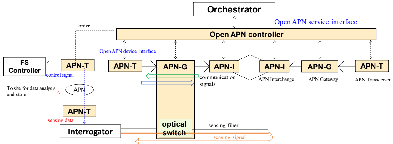
Figure 6-1 System control for telemetry
