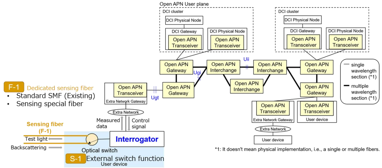
Figure 1-1 Fiber sensing architecture Type I
