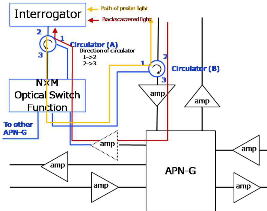
Figure 4-5 Configuration using circulator where backscattered light is inserted into APN-G through the circulator
