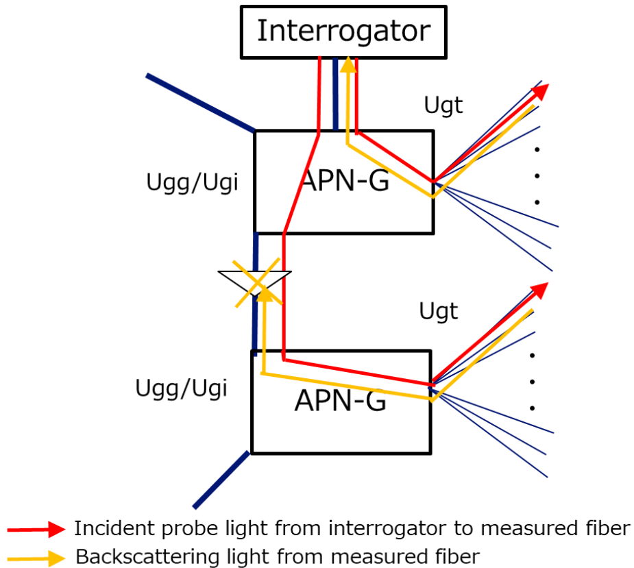
Figure 4-2 Probe light from the interrogator to pass through multiple APN-Gs
