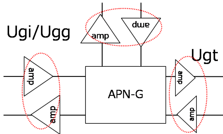
Figure 4-1 APN-G configuration with amplification
