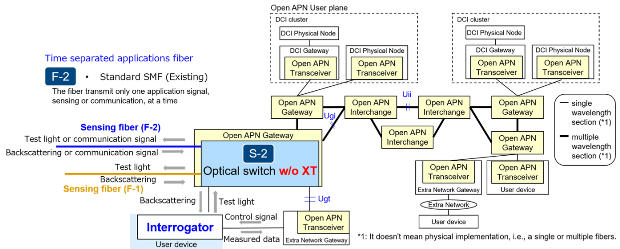
Figure 1-2 Fiber sensing architecture Type II-1
