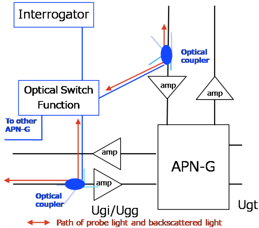
Figure 4-6 Configuration with couplers
