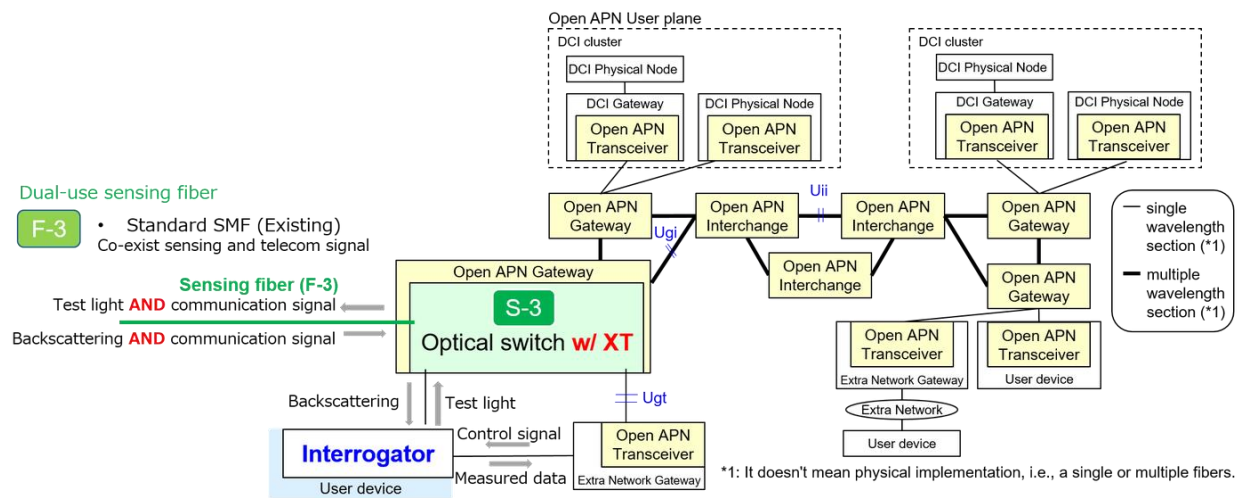
Figure 1-4 Fiber sensing architecture Type III
