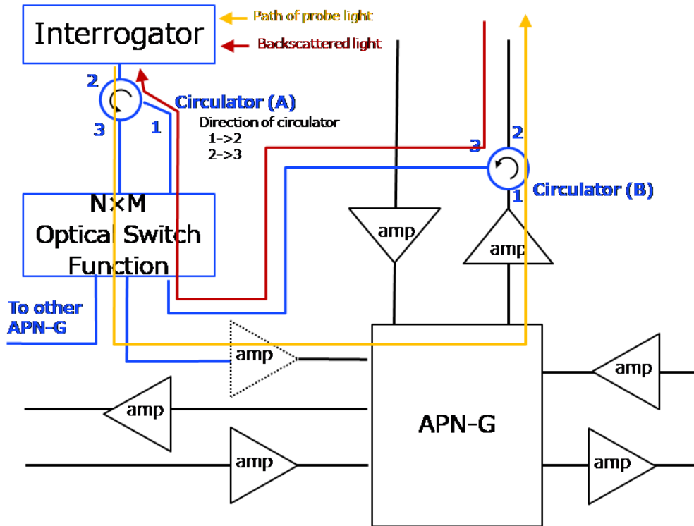
Figure 4-4 Configuration using circulator where backscattered light is inserted into APN-G through the circulator
