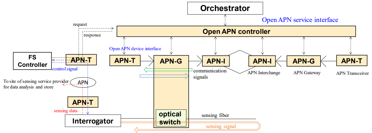
Figure 6-2 System control for environmental sensing
