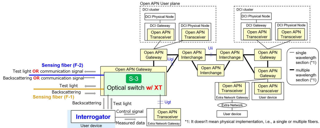
Figure 1-3 Fiber sensing architecture Type II-2
