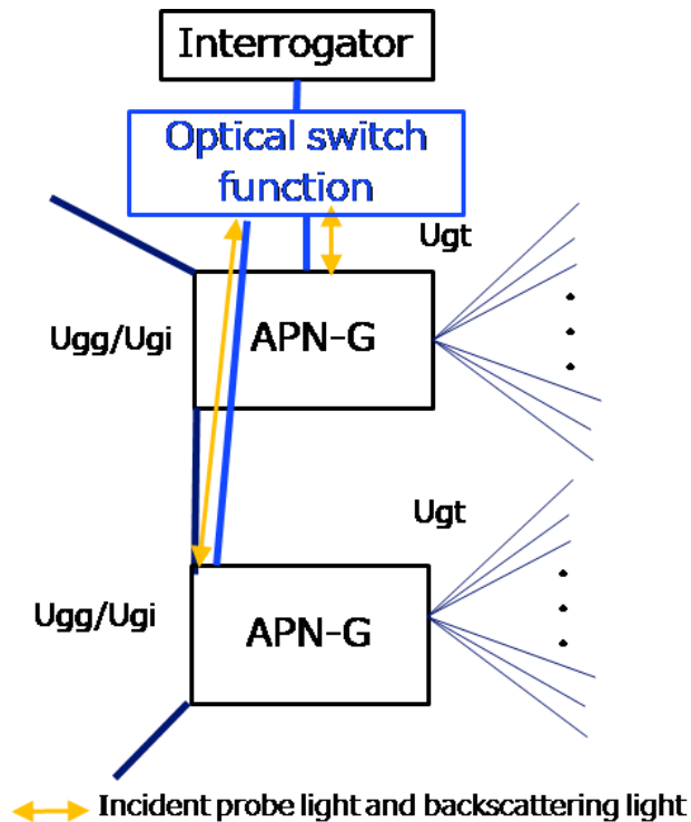
Figure 4-3 External switch dedicated to fiber sensing in the first stage for selecting each APN-G
