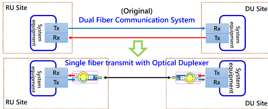
Figure 19 Single-fiber bidirectional access architecture
