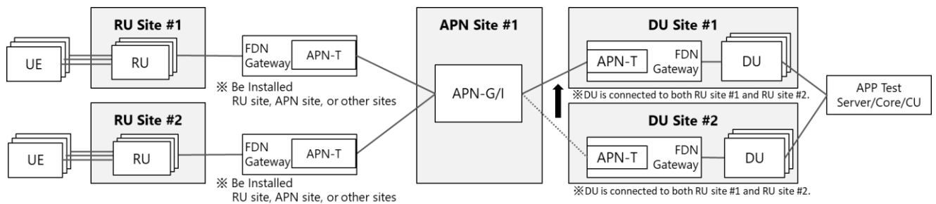
Figure 11 PtMP topology of the deployment scenario in Step 2
