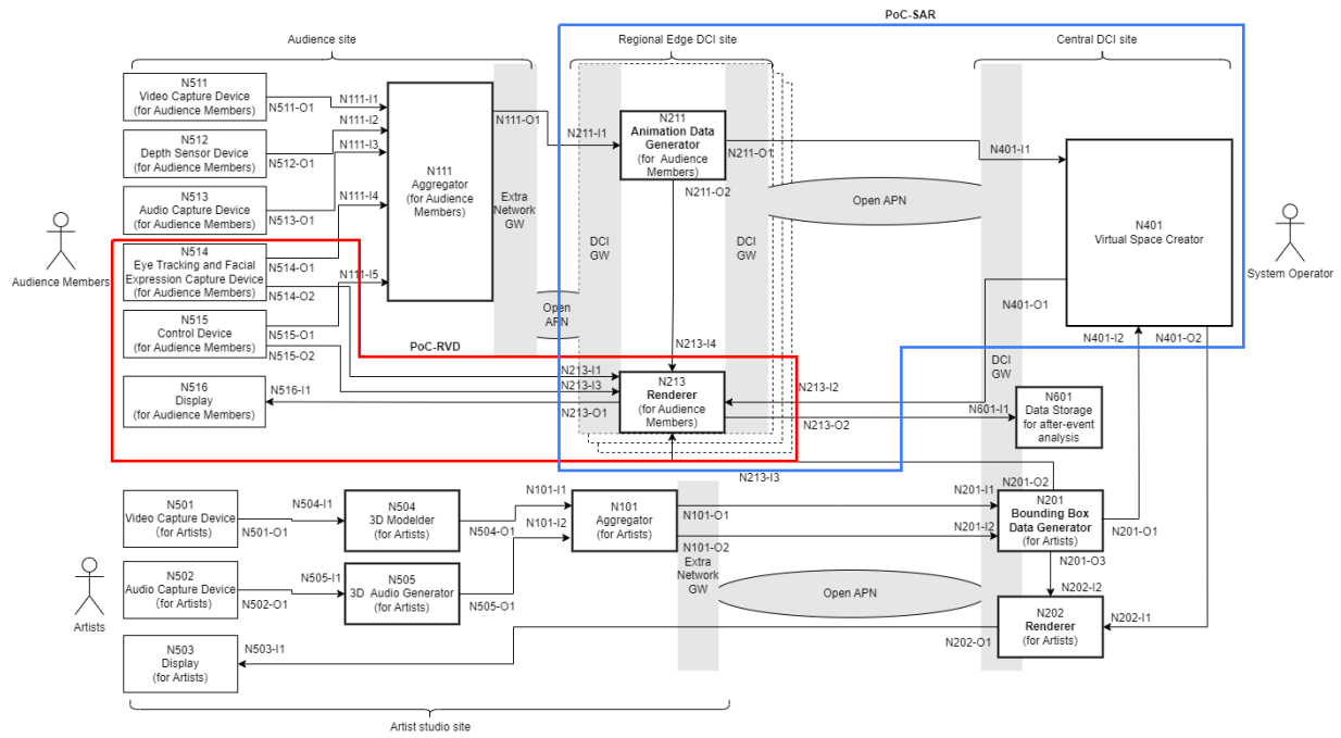
Figure 1.3-1: Scopes of PoCs to evaluate the ILM RIM
