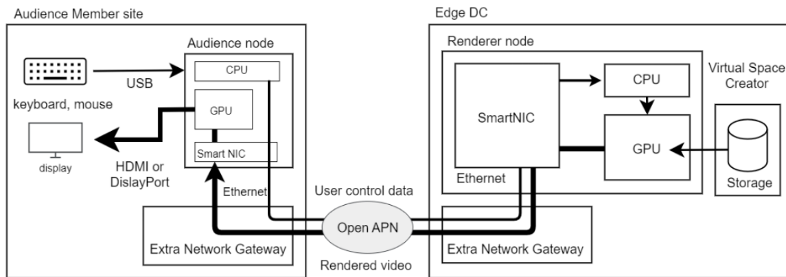
Figure A-1: An Implementation Example with RDMA
