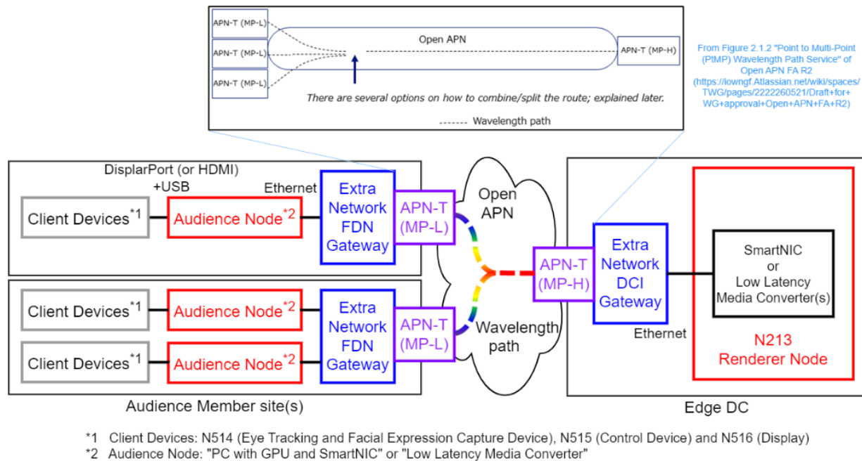
Figure 2.1-3: Example of the Open APN PtMP and FDN Functional Architecture between Renderer Node in Edge DC and Audience Node in Audience Member Site(s)
