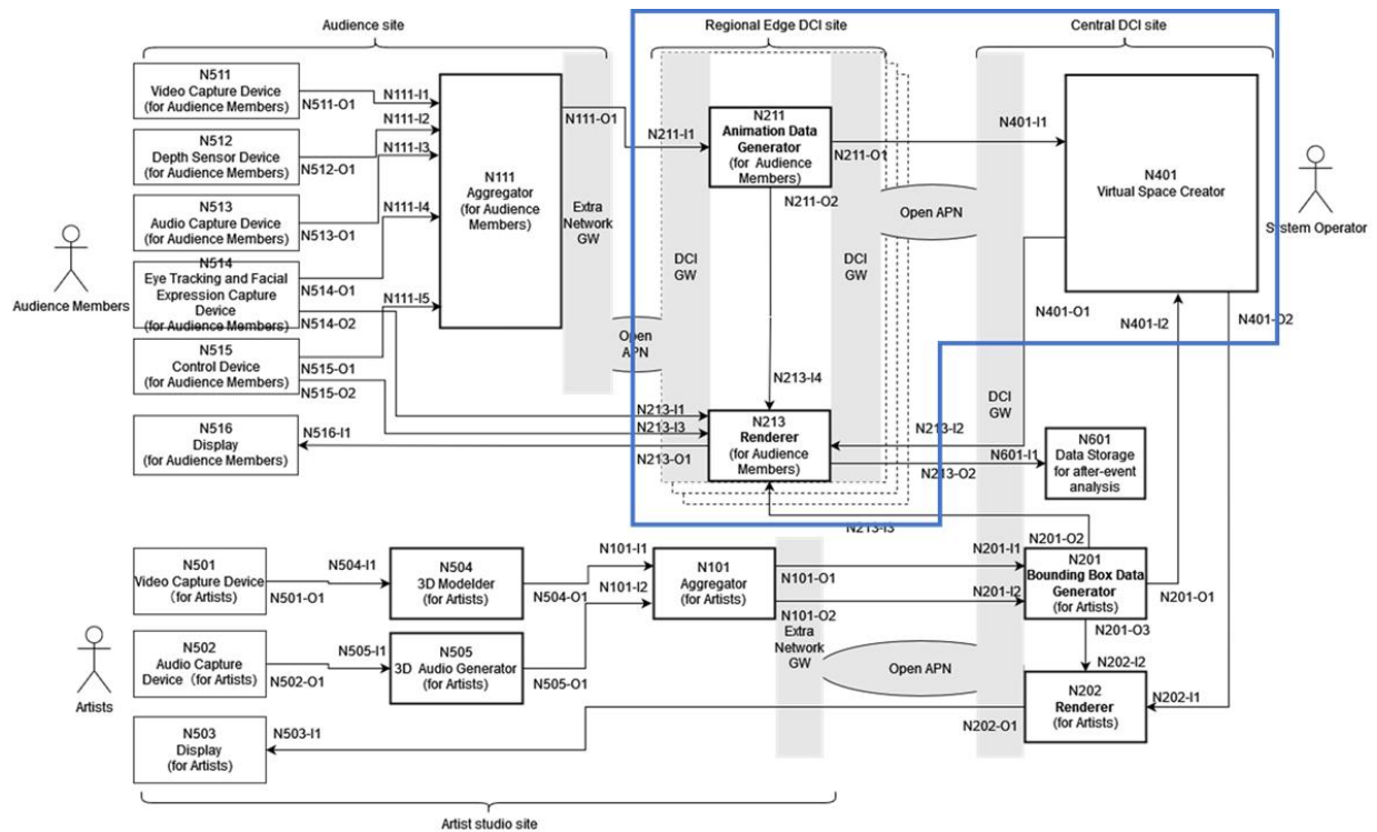
Figure 2.2-1: Overview of PoC-SAR
