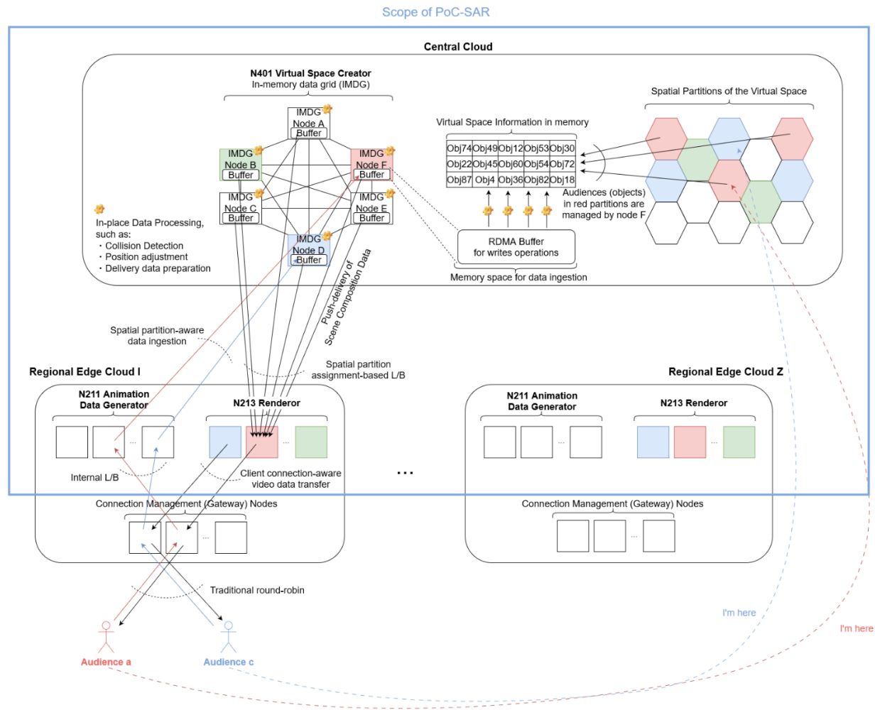
Figure 2.2-2: Assumed Physical Configuration of PoC-SAR
