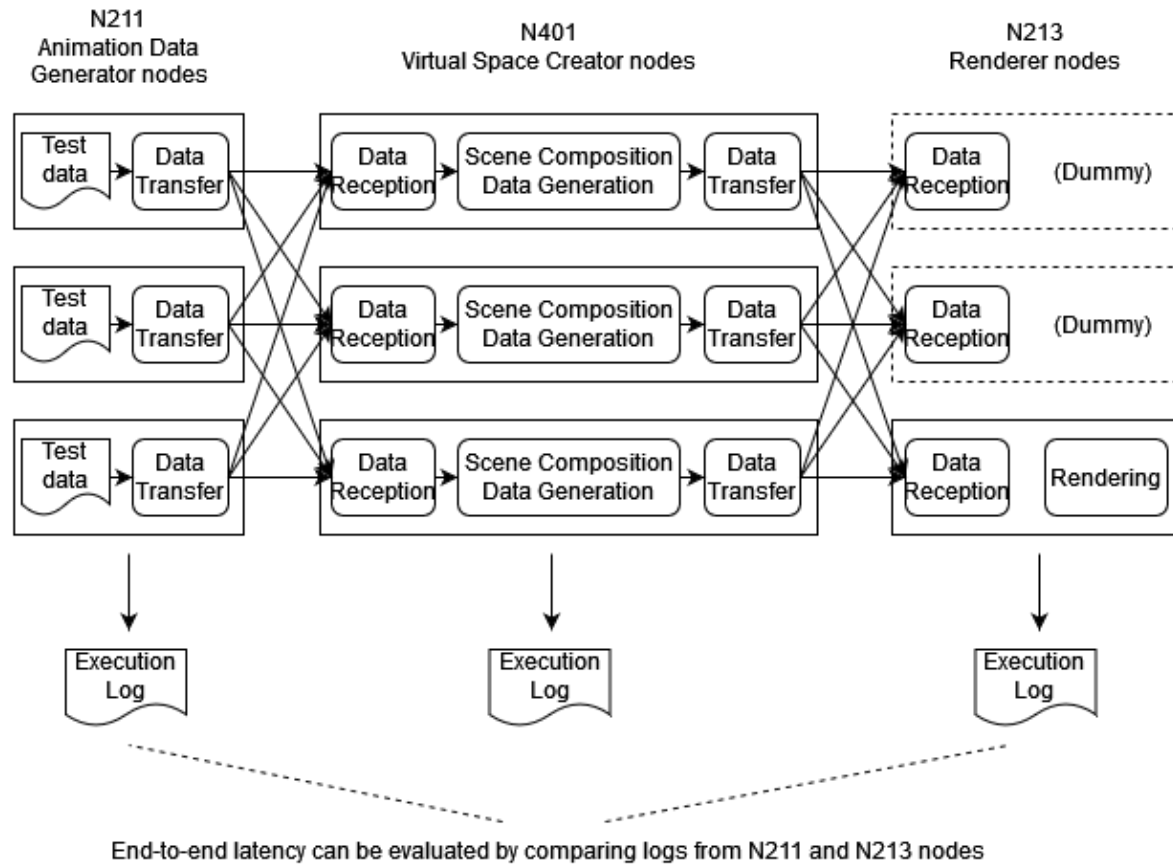
Figure 2.2-3: Assumed Physical Configuration of N211, N213, and N401 Nodes in PoC-SAR
