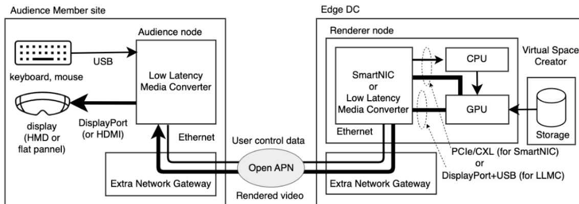
Figure A-2: Implementation Example with RTP
