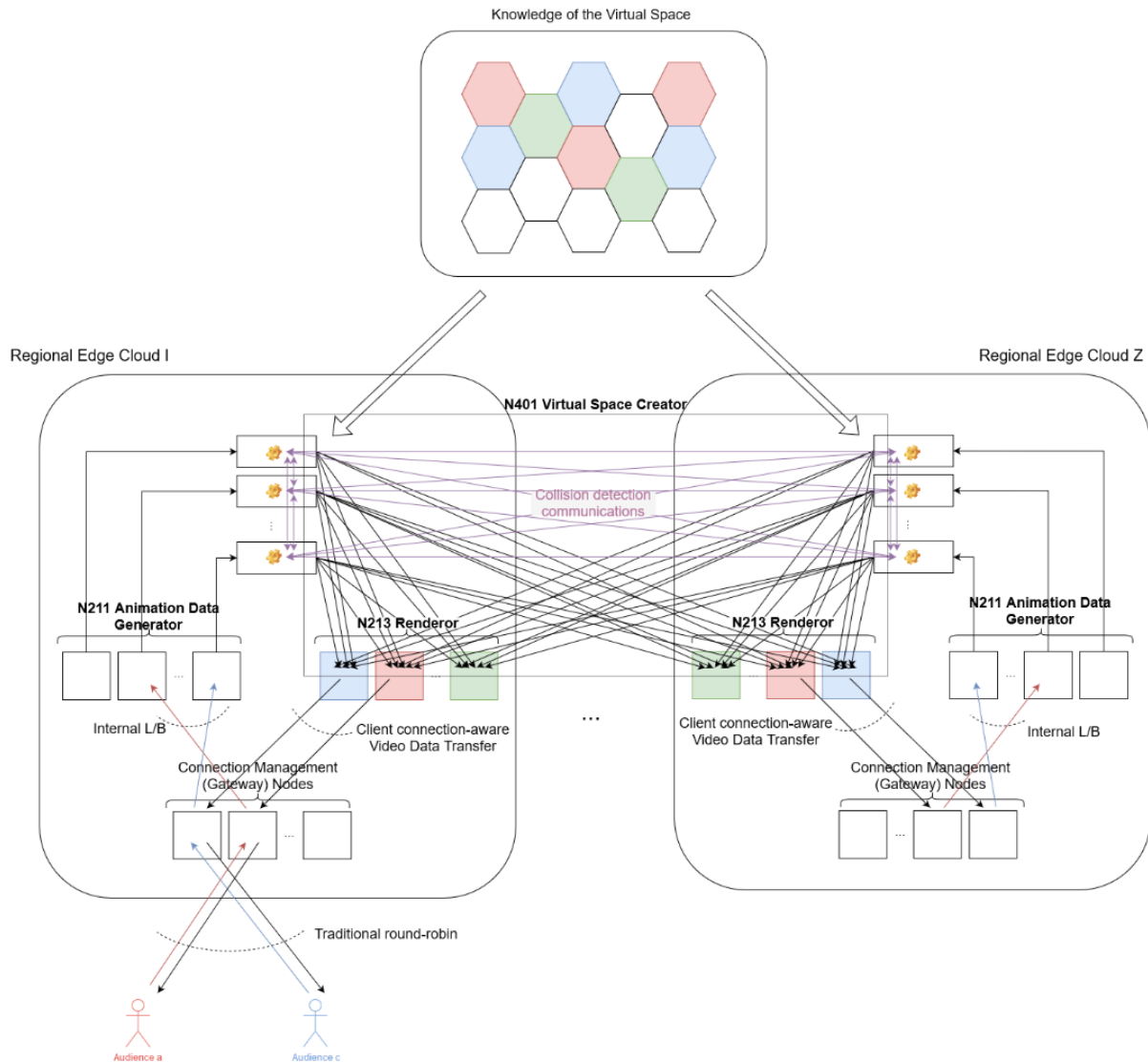
Figure C.1-1: Geo-Distributed Implementation of the Virtual Space Creator
