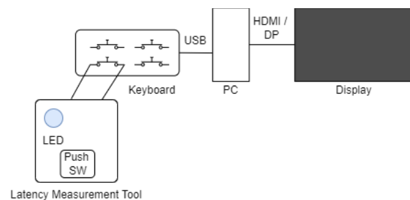
Figure B.2-1: Overview of the Latency Measurement System
