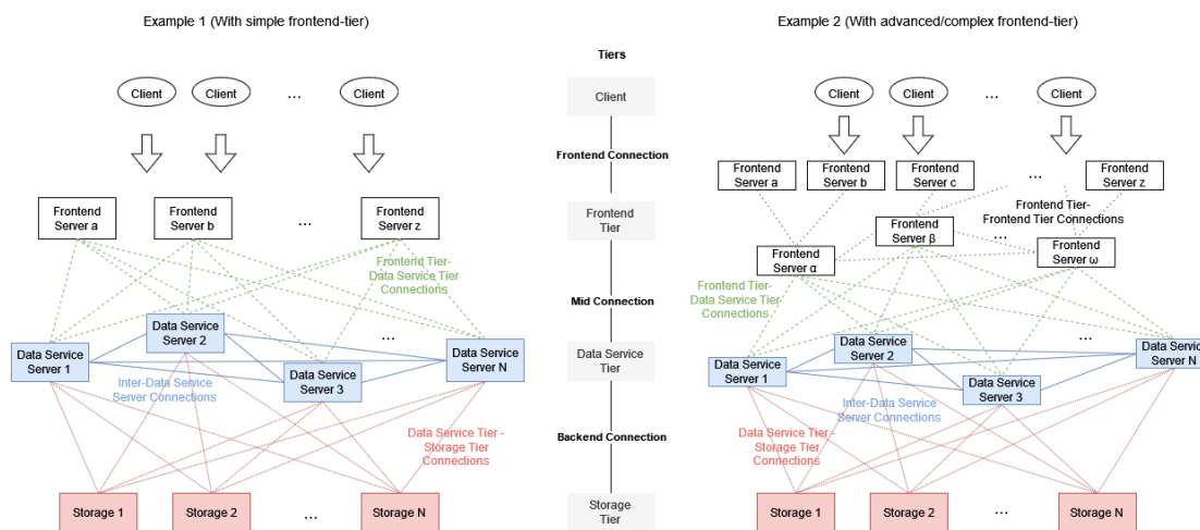
Figure 5-1-2, Connection Patterns between the IDH Components
