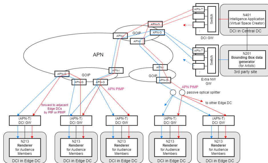
Figure A-17: Some potential approaches for multicast over APN
