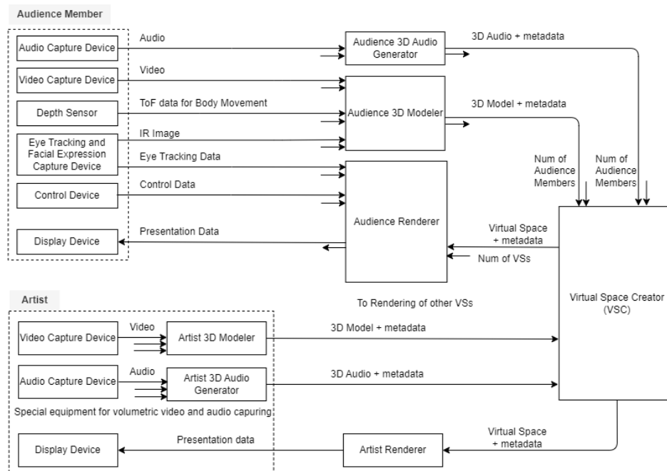
Figure 2.1-1: System Overview
