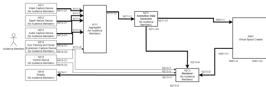
Figure 3.2-3: Sending Animation Data
