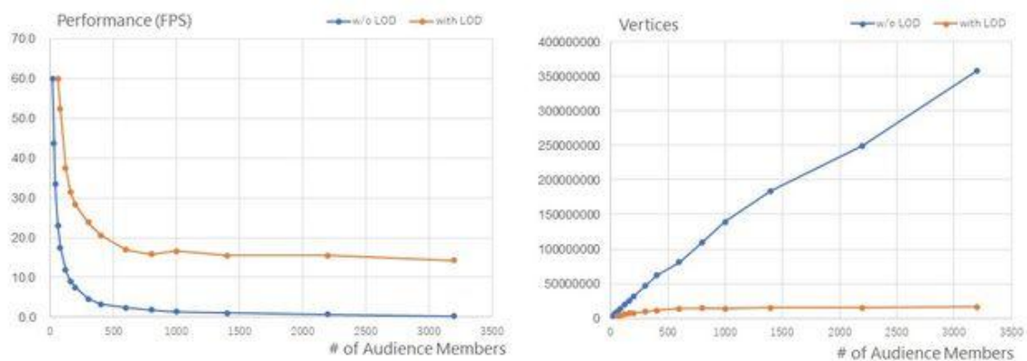
Figure A-36: The Effects of LOD
