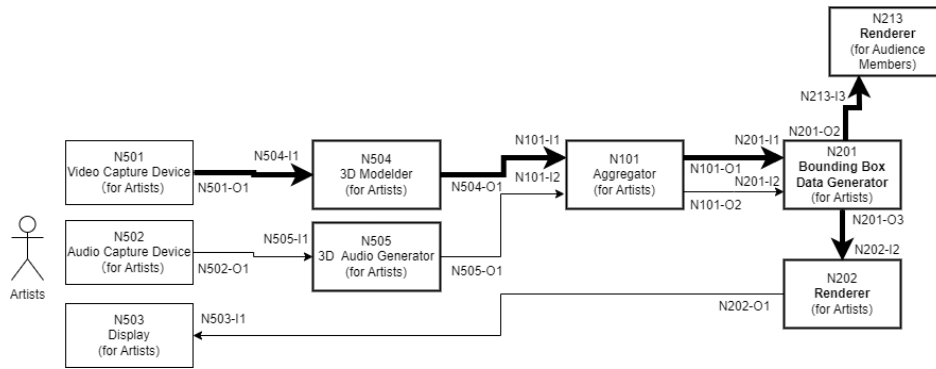
Figure 3.2-2: Sending volumetric video data
