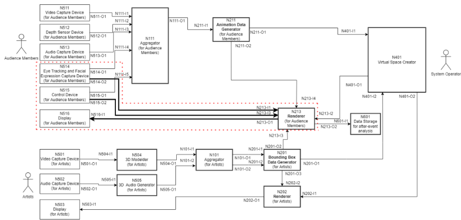
Figure 3.1-3: Transmission of the Animation Data to Virtual Space Creator and Avatar Data to the Renderer
