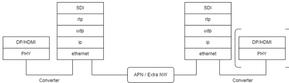
Figure A-21: Protocol Stack of SDI over IP (ST2202)
