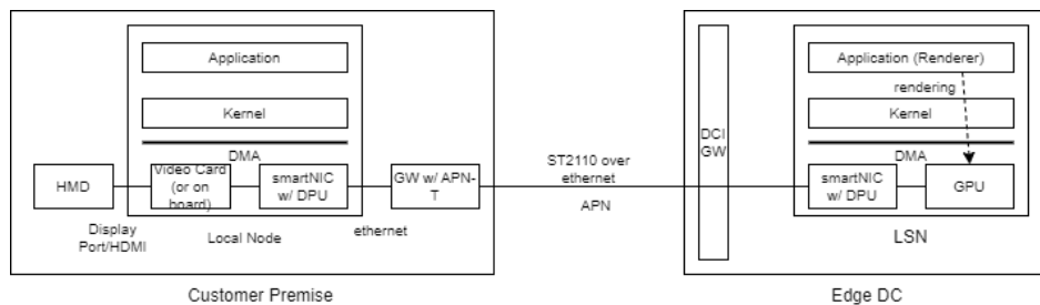
Figure A-22: An example of system structure of SDI over IP (ST2110)
