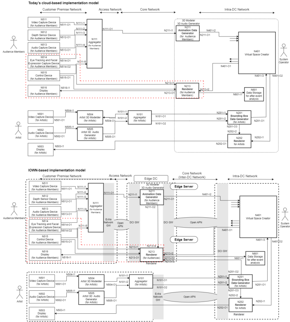
Figure 5.4-1: Today's centralized implementation model and IOWN GF-based RIM
