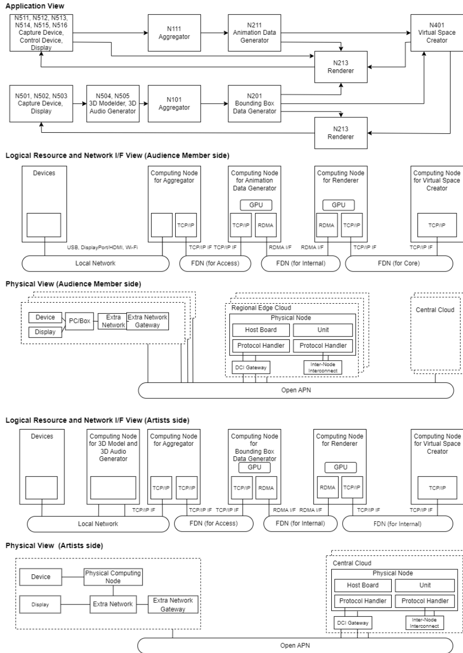
Figure 5.2-1: Overview of an IOWN GF-Based RIM, Application View
