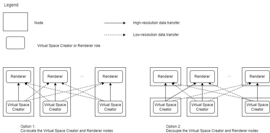
Figure A-38: System topology options around the Virtual Space Creator and the renderer nodes
