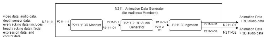
Figure A-11: Animation Data Generator for Audience Members
