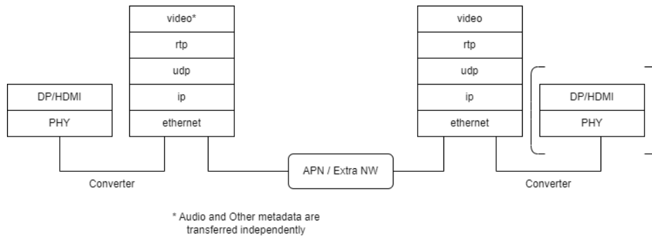
Figure A-23: Protocol Stack of SDI over IP (ST2110)
