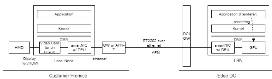
Figure A-20: An example of system structure of SDI over IP (ST2202)
