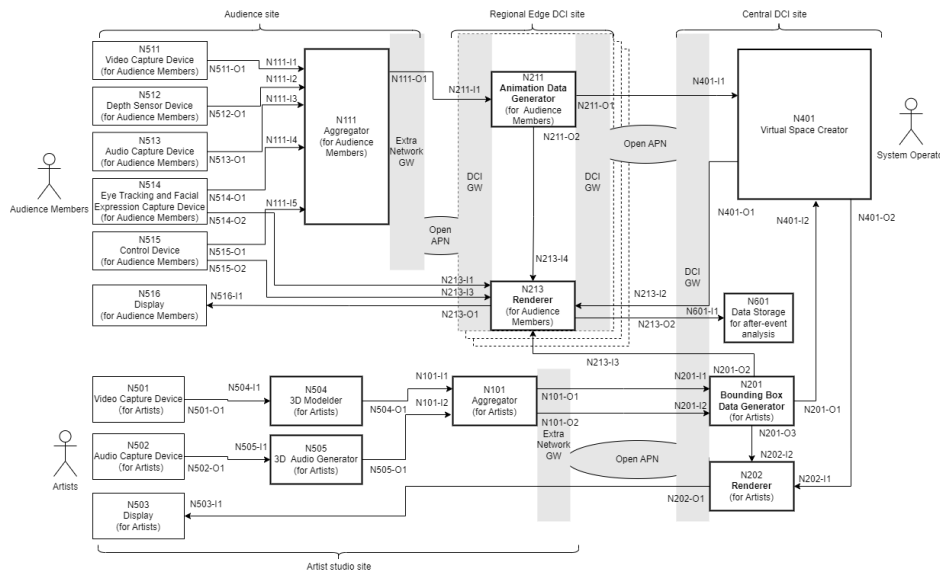
Figure 5.2-2: Overview of an IOWN GF-Based RIM
