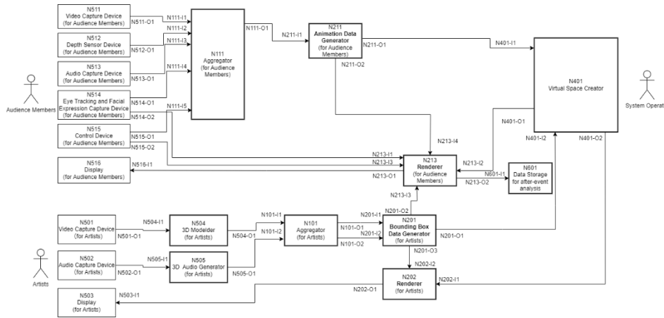
Figure A-4: A Data Pipeline Diagram for the Interactive Music Use Case (same as Figure 3.1-1)
