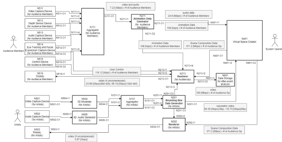
Figure 3.2-1: Summary of the primary dataflow
