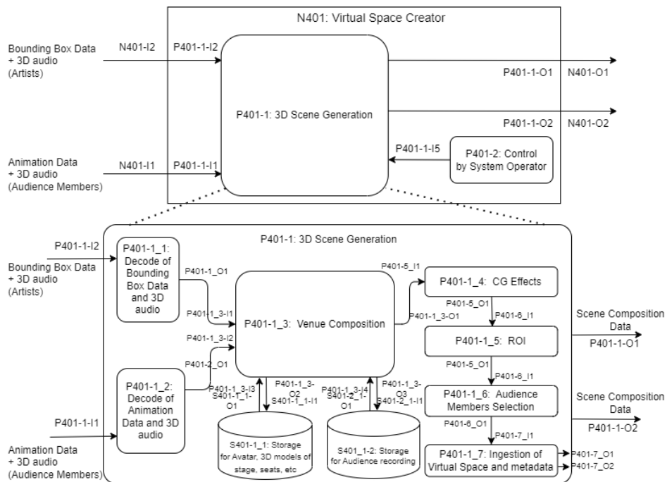
Figure A-7: N401 Virtual Space Creator
