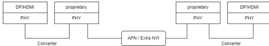
Figure A-25: Example of Protocol Stack of DisplayPort/HDMI over APN
