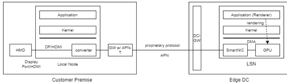
Figure A-24: An example of system structure of DisplayPort/HDMI over APN
