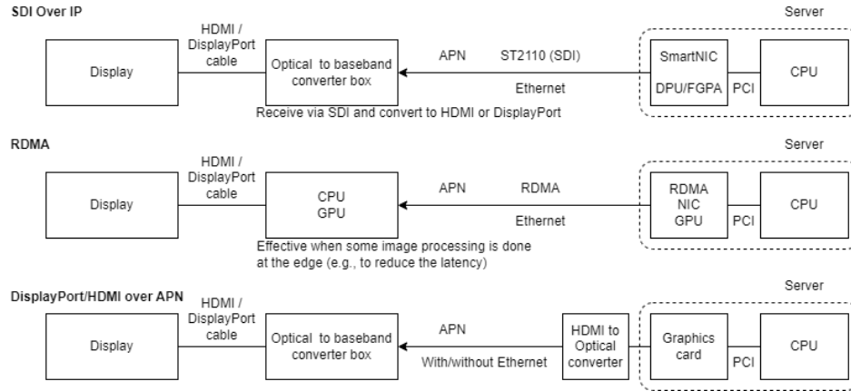
Figure 5.2-5: Communication between the Renderer node and the Display of customer premise
