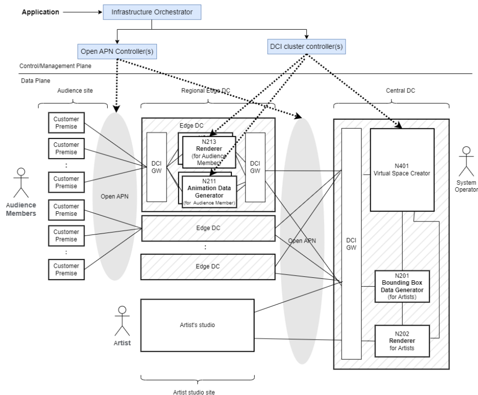
Figure 5.2-3: Dynamic resource allocation by Infrastructure Orchestrator
