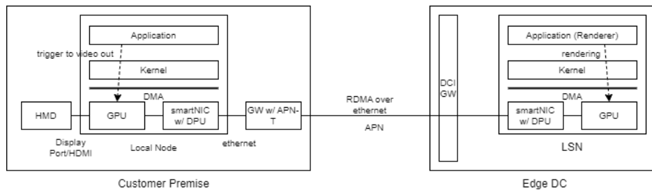
Figure A-18: An example of system structure of RDMA (RoCE v2)
