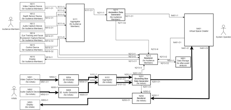
Figure 3.1-2: Transmission of 3D model data and 3D audio data
