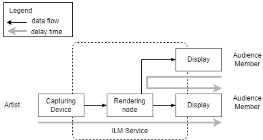
Figure 2.5-1: Data stream toward Audience Members
