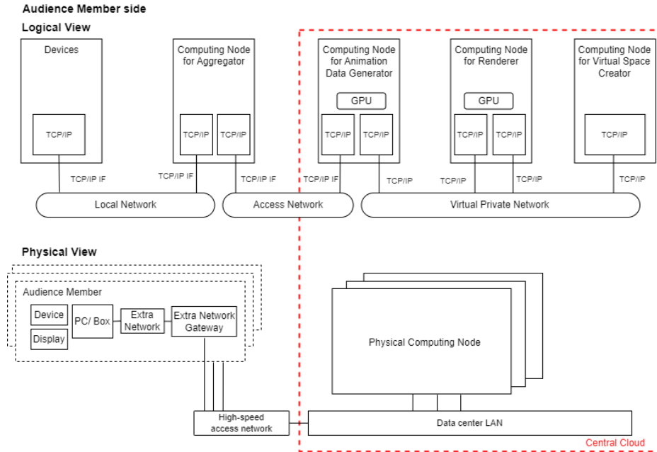
Figure 4.1-2: Today's Centralized Cloud-Based Implementation (Audience Member side)
