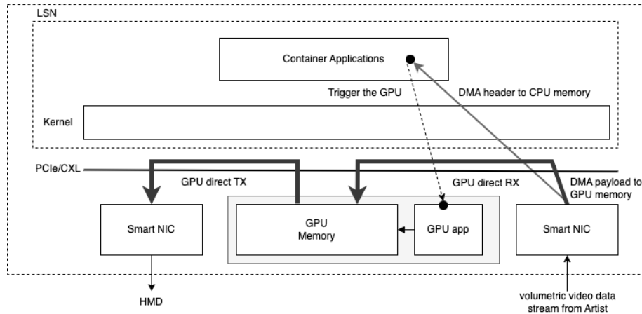
Figure 5.3-1: Example of communication between Renderer and Display
