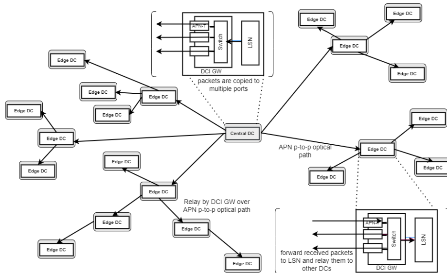
Figure 5.2-4: Example of multicast over APN from central data center to edge data centers
