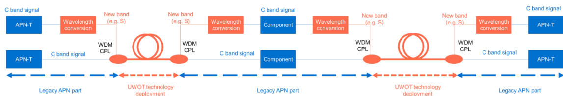
Figure 7-1-1: Hybrid deployment of new bands
