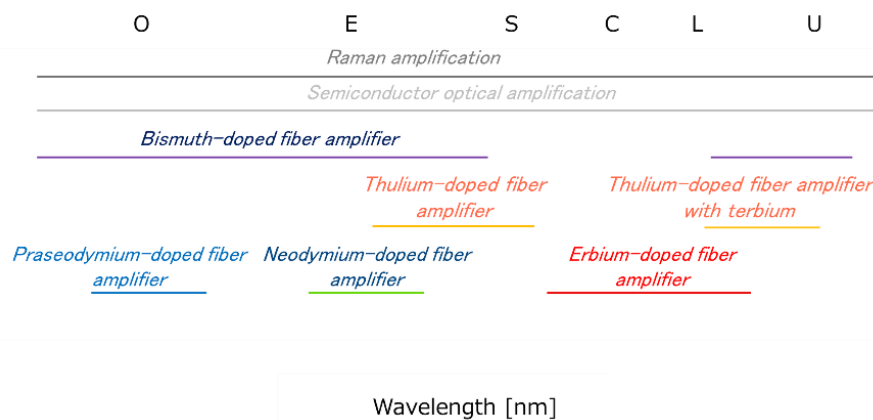
Figure 3-3-1: Amplification technologies over wide-band spectrum
